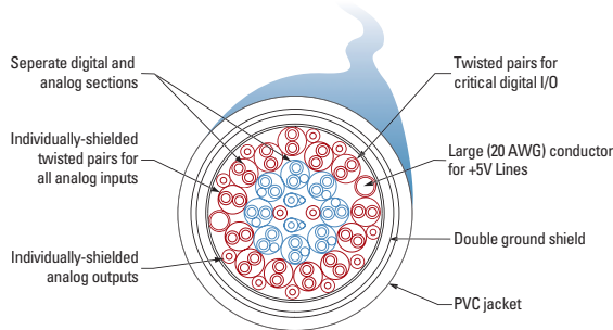
Figure 1. SH68-68-EP Cable
